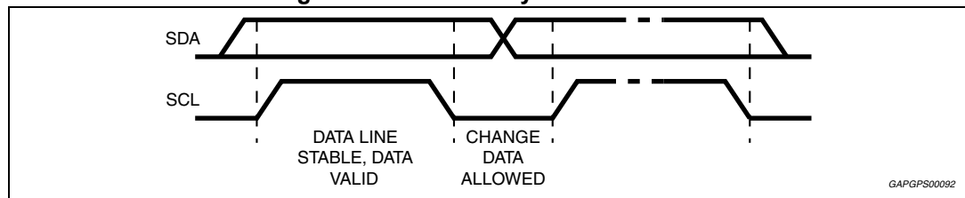
Figure 30. Timing diagram on the I 2 C bus
