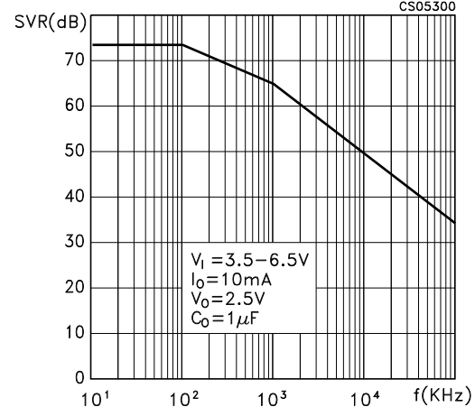
Figure 12. Supply voltage rejection vs. frequency (Co = 1 µF)
