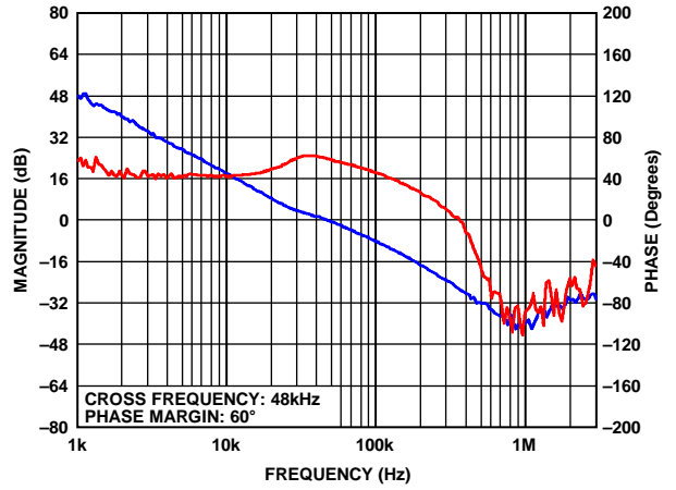
Figure 48. ADP2120 Bode Plot at V_{IN} = 5\text{ V} , V_{OUT} = 3.3\text{ V} , I_O = 1.25\text{ A} , L = 2.2\ \mu\text{H} , C_{OUT} = 2 \times 10\ \mu\text{F}
