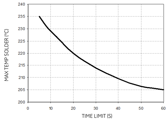
Figure 33. Time Limit Curve Above 205°C Reflow.
