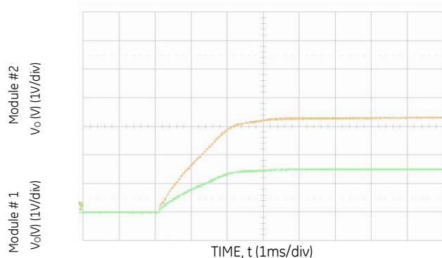
Figure 13. Synchronized Start-up of Output Voltage when SEQ/ENA pins are tied together (Module #1 = 1.5Vdc, Module #2 = 3.3Vdc).
