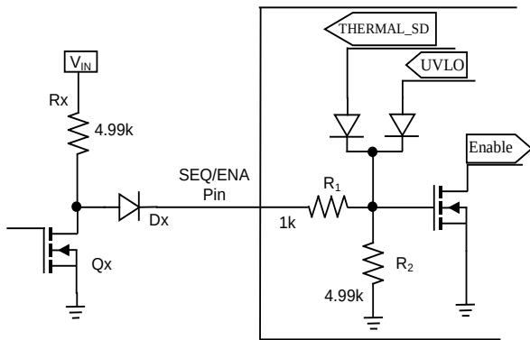
Figure 25. Remote On/Off Implementation.
