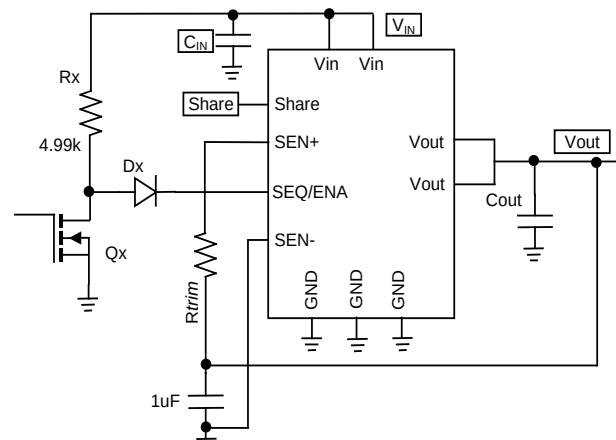
Figure 24. Application Schematic
