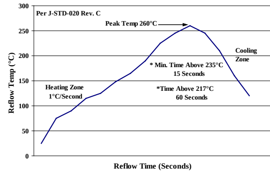
Figure 34. Recommended linear reflow profile using Sn/Ag/Cu solder.
