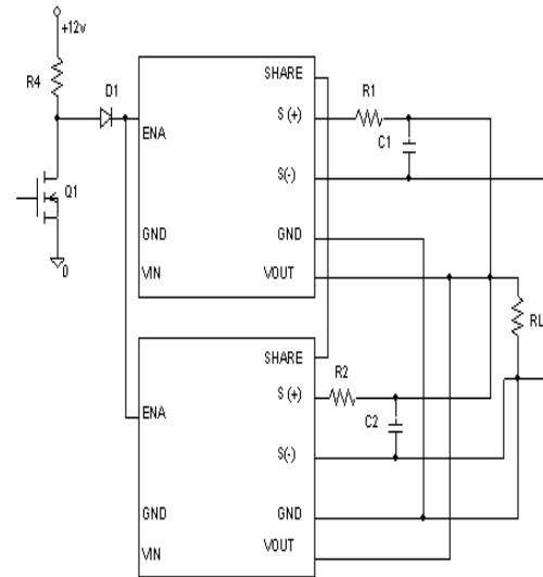
Figure 28. Circuit Configuration for modules in parallel.
