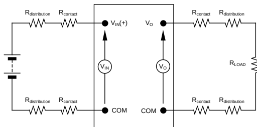
Figure 22. Output Ripple and Noise Test Setup.
