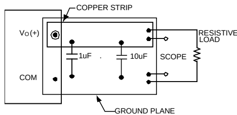
Figure 21. Input Reflected Ripple Current Test Setup.
