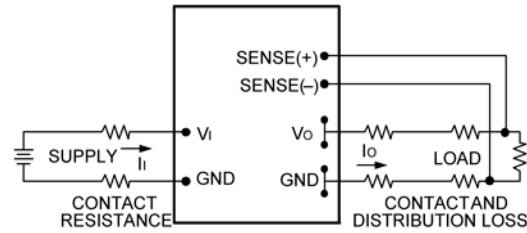
Figure 26. Effective Circuit Configuration for Remote sense operation
