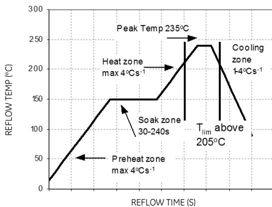
Figure 32. Recommended Reflow Profile.
