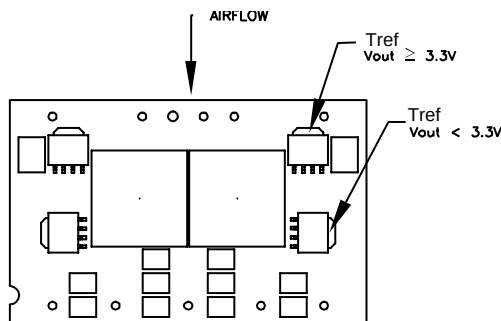
Figure 29. T_{ref} Temperature measurement location.
