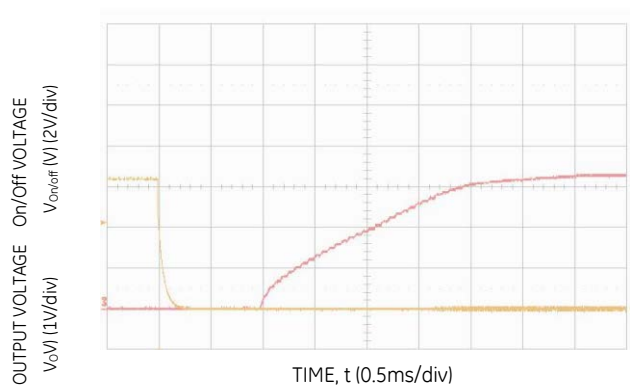
Figure 12. Typical Start-Up Using Enable ( V_o = 3.3V dc).
