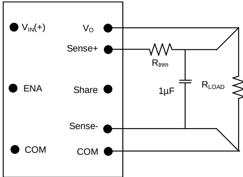
Figure 27. Circuit Configuration for Programming
