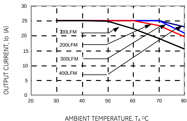
Figure 17. Derating Output Current versus Local Ambient Temperature and Airflow ( V_{in} = 12Vdc , V_o = 3.3 Vdc ).
