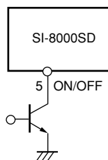
V_{OUT} . ON/OFF
