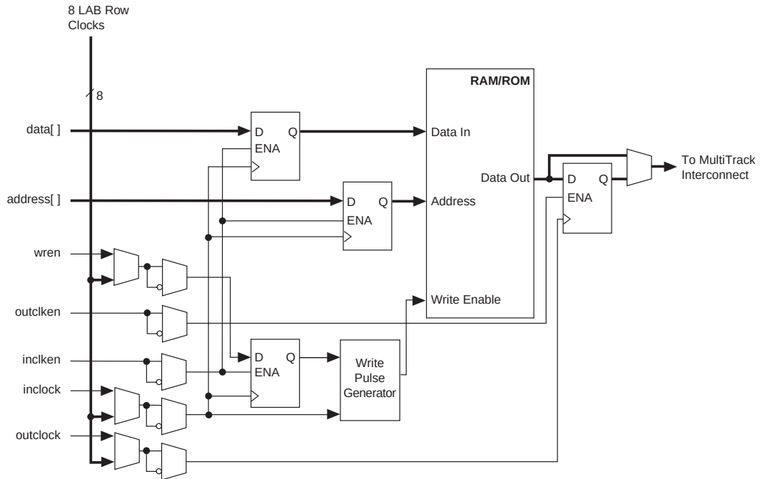
Figure 14–13. Single-Port Mode Notes (1), (2), (3)
