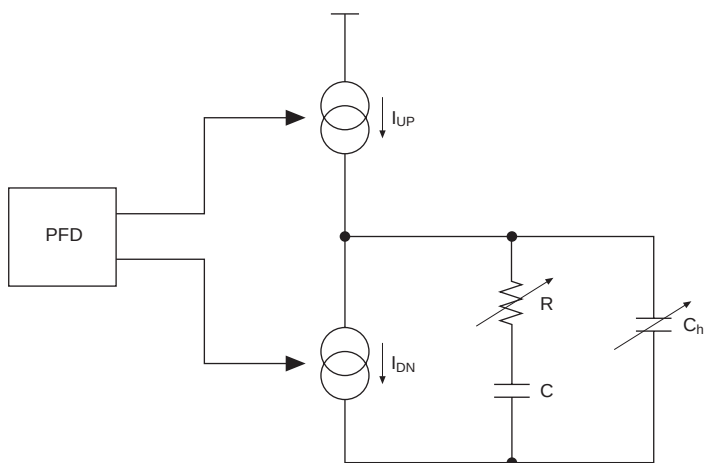
Figure 13–13. Loop Filter Programmable Components
