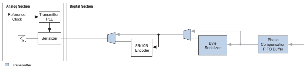
Figure 4–9. Block Diagram of the Transmitter Digital Components in SONET Mode
