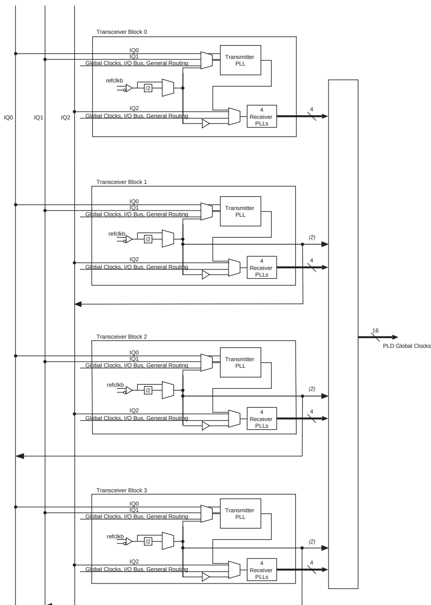
Figure 3–23. Inter-Transceiver Line Connections for EP1SGX25 Device
