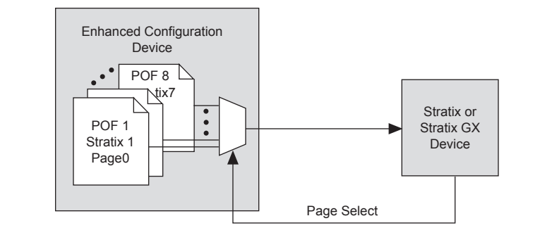
Figure 2–5. Page Mode Feature in Stratix or Stratix GX Devices & Enhanced Configuration Devices
