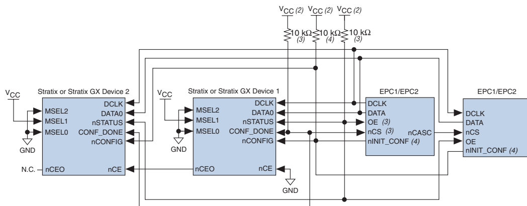
Figure 1–3. Multi-Device Configuration Circuit Note (1)
