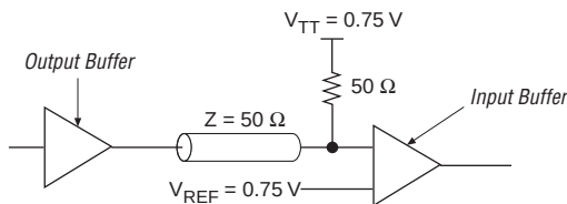
Figure 16–1. HSTL Class I Termination
