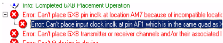
Figure 12–2. Error Messages
