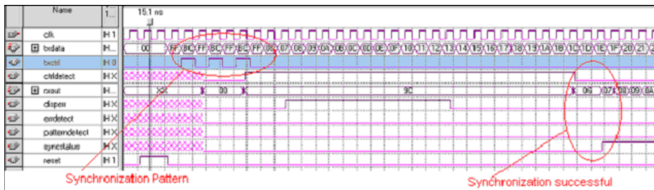
Figure 6–37. GIGE Synchronization Sequence Quartus II Software Simulation Results
