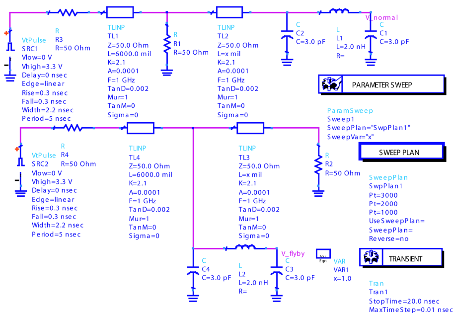
Figure 4–58. ADS Simulation Setup for Normal Versus Fly-By Termination
