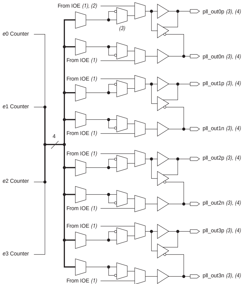
Figure 13–5. External Clock Outputs for PLLs 5 & 6
