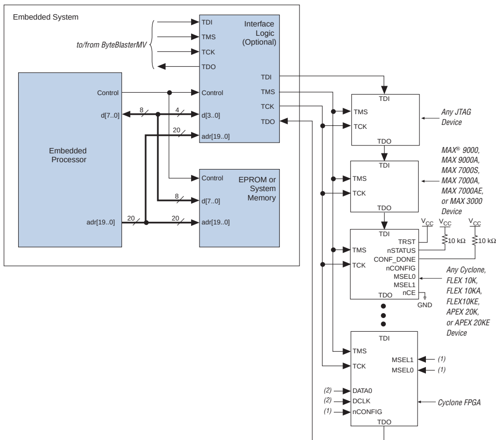
Figure 1–23. Embedded System Block Diagram
