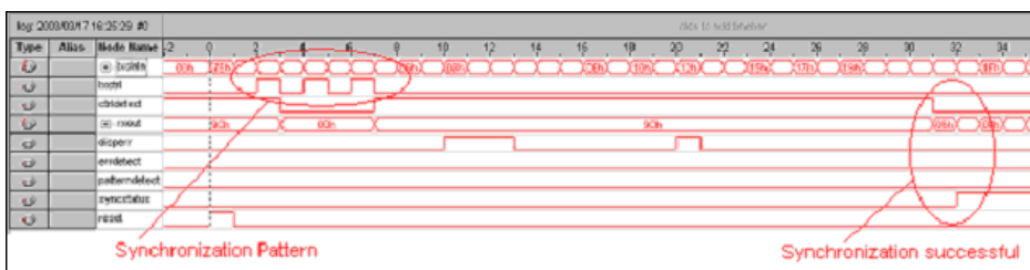
Figure 6–36. GIGE Synchronization Sequence SignalTap II Results
