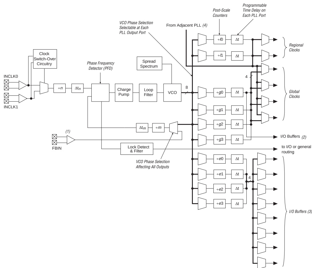
Figure 13–3. Stratix & Stratix GX Enhanced PLL
