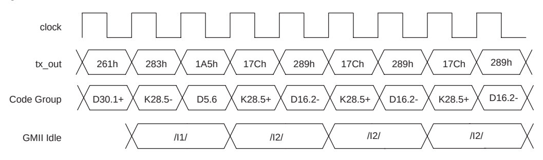
Figure 6–8. Idle Generation With /I1/ Ordered Set
