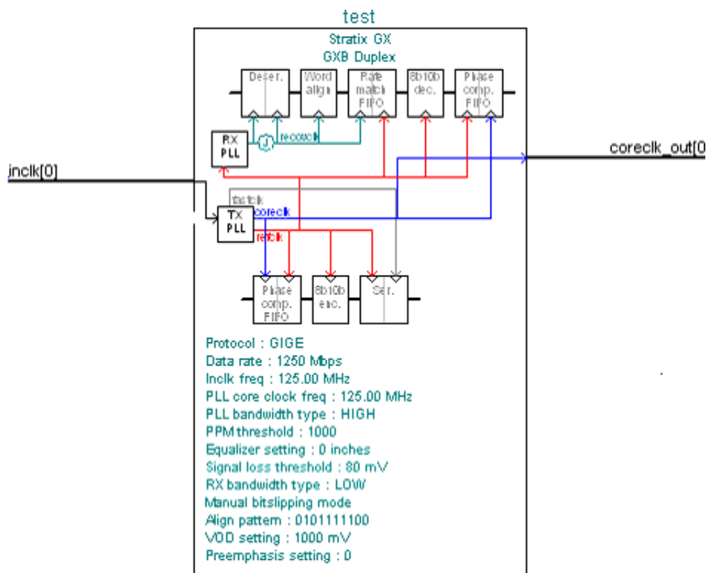
Figure 6–21. Default Configuration of altqxb Megafunction in GIGE Mode
