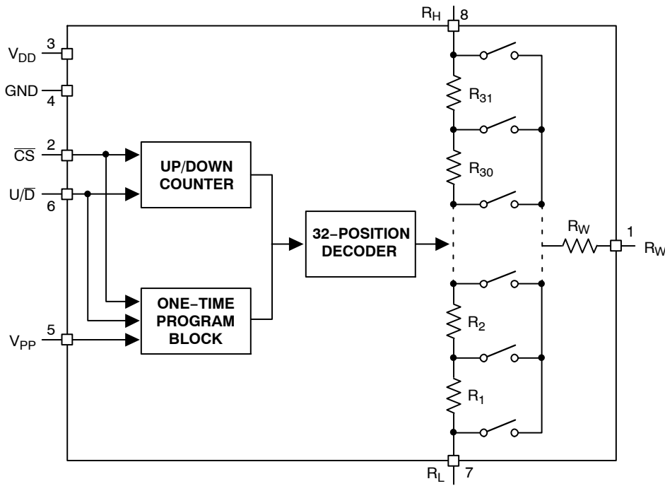
Figure 1. Functional Diagram
