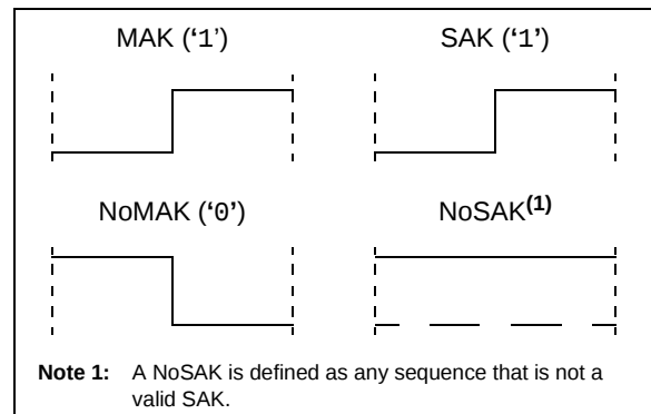
FIGURE 5-3: ACKNOWLEDGE BITS
