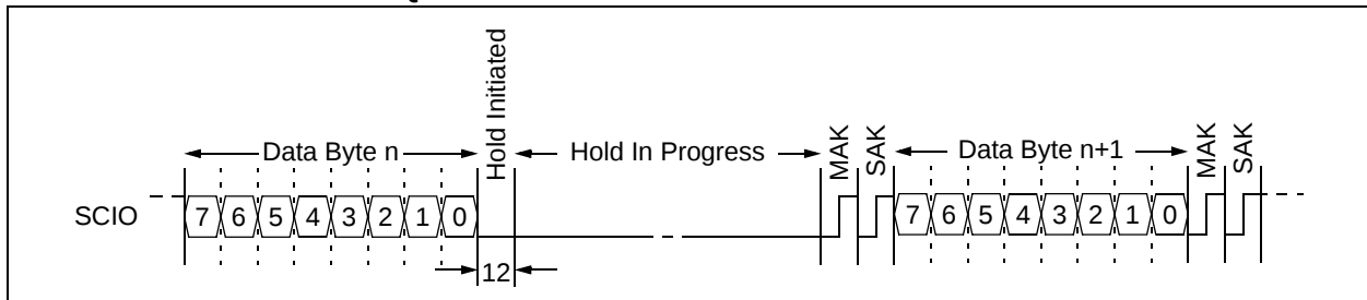
FIGURE 12-5: HOLD SEQUENCE
