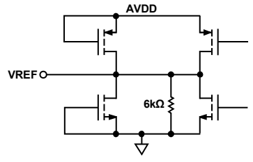
Figure 75. Equivalent VREF Circuit
