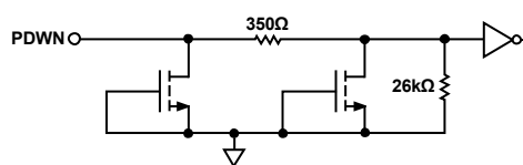
Figure 76. Equivalent PDWN Input Circuit
