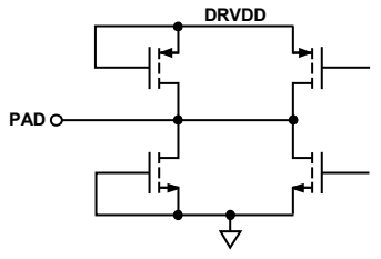
Figure 70. Digital Output
