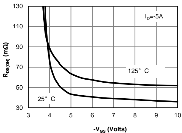
Figure 16: On-Resistance vs. Gate-Source Voltage
