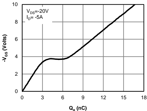
Figure 18: Gate-Charge Characteristics
