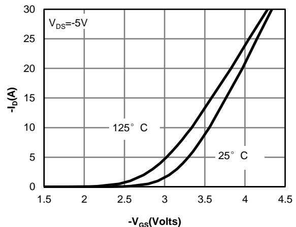
Figure 13: Transfer Characteristics
