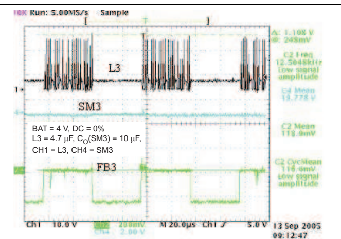
Figure 57. SM3 Led Current vs PWM Duty Cycle
