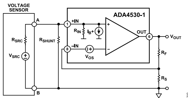
Figure 105. Voltage Buffer Circuit
