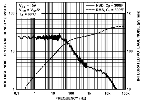
Figure 132. RTO Noise Spectral Density (60°C)
