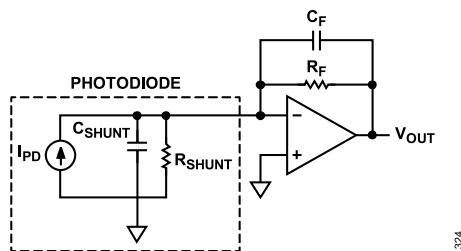
Figure 125. Transimpedance Amplifier with Photodiode Model
