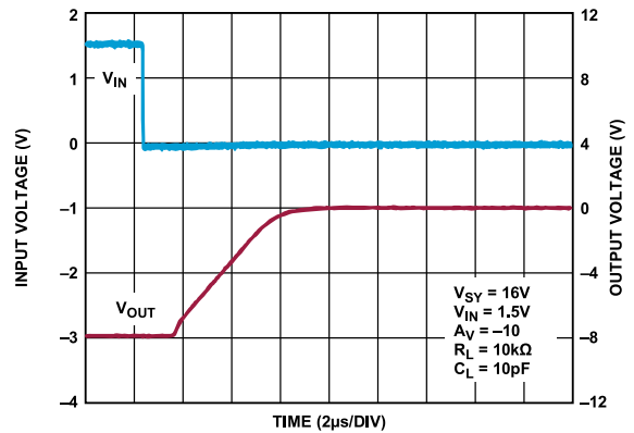
Figure 72. Negative Overload Recovery, V_{SY} = 16\text{ V}
