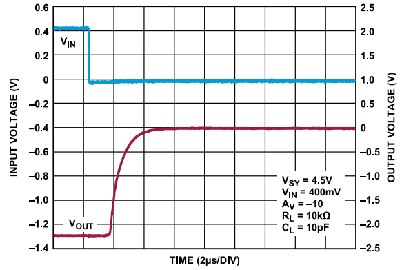
Figure 70. Negative Overload Recovery, V_{SY} = 4.5\text{ V}
