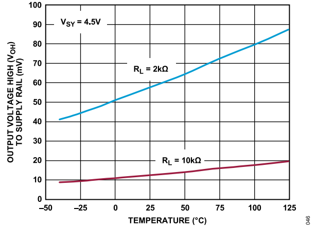
Figure 49. Output Voltage High ( V_{OH} ) to Supply Rail vs. Temperature, V_{SY} = 4.5\text{ V}
