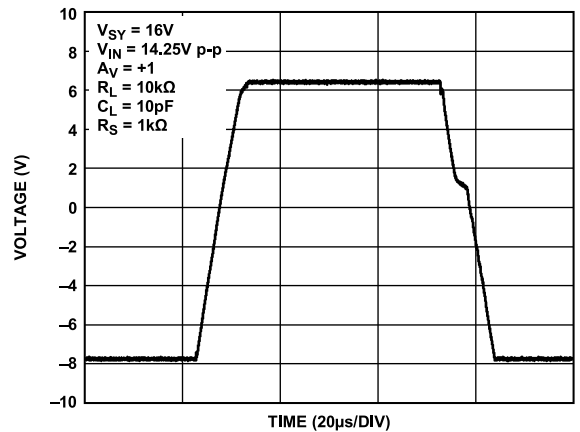
Figure 66. Large Signal Transient Response, V_{SY} = 16\text{ V}
