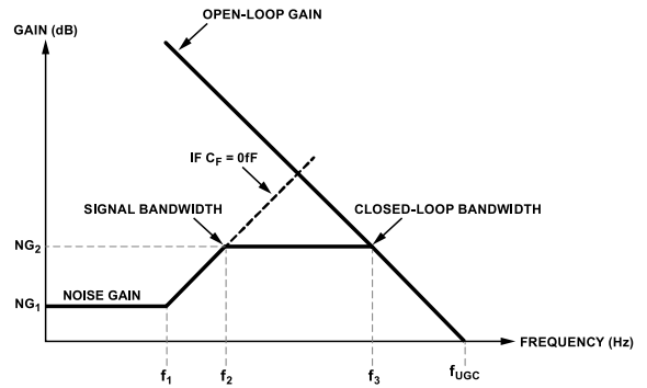
Figure 126. Transimpedance Noise Gain vs. Frequency
