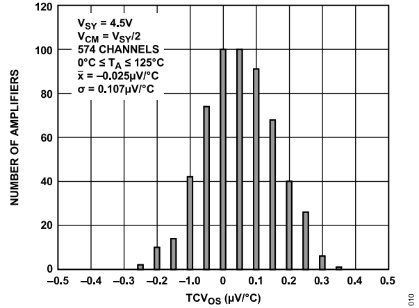
Figure 13. Input Offset Voltage Drift Distribution, 0^{\circ}\text{C} \leq T_A \leq 125^{\circ}\text{C} , V_{SY} = 4.5 V
