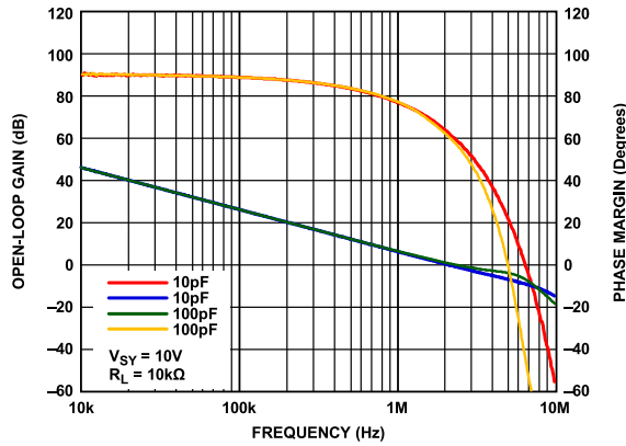
Figure 55. Open-Loop Gain and Phase Margin vs. Frequency
