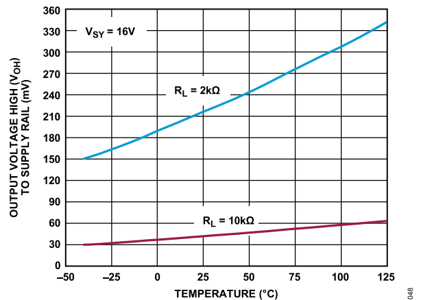
Figure 51. Output Voltage High ( V_{OH} ) to Supply Rail vs. Temperature, V_{SY} = 16\text{ V}
