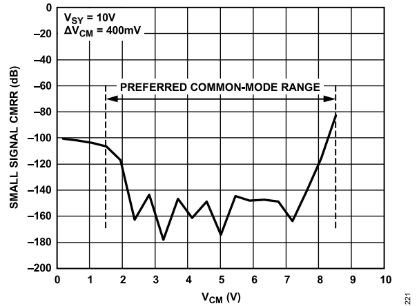
Figure 21. Small Signal CMRR vs. Common-Mode Voltage ( V_{CM} )
