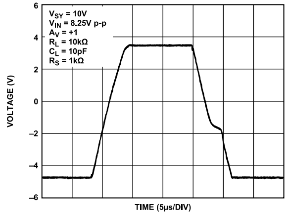
Figure 65. Large Signal Transient Response, V_{SY} = 10\text{ V}
