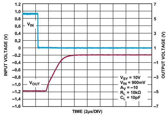
Figure 71. Negative Overload Recovery, V_{SY} = 10\text{ V}
