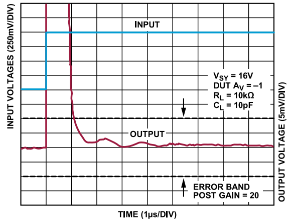
Figure 78. Positive Settling Time to 0.1%, V_{SY} = 16V
