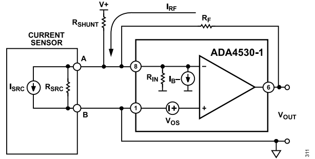
Figure 106. TIA Circuit
