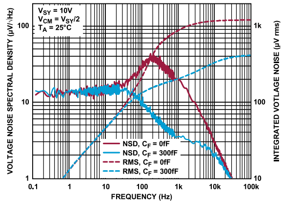
Figure 131. RTO Noise Spectral Density (25°C)
