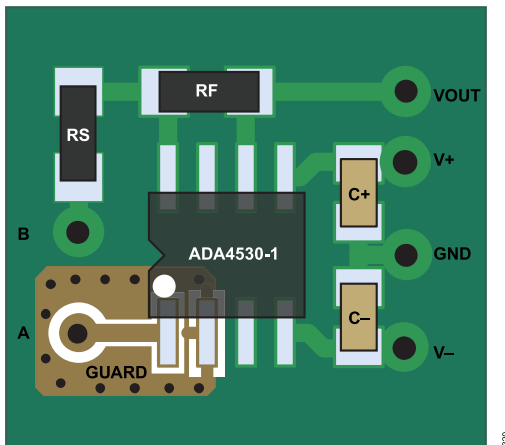
Figure 121. Buffer Circuit Layout
