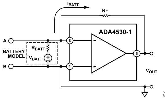
Figure 115. TIA Circuit with Contamination Battery
