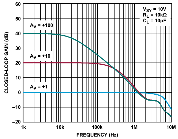
Figure 58. Closed-Loop Gain vs. Frequency
