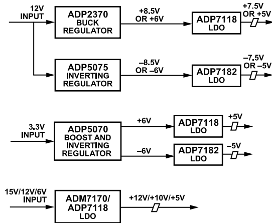
Figure 133. Recommended Power Solutions
