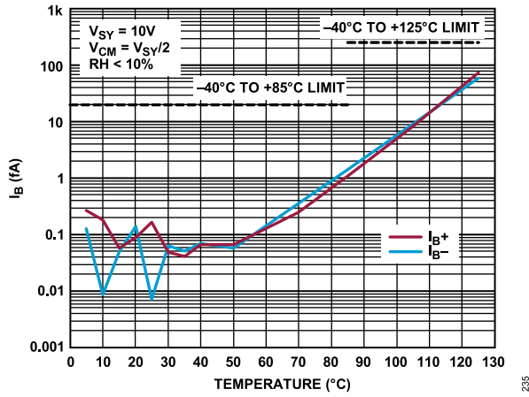
Figure 35. Input Bias Current ( I_B ) vs. Temperature, V_{SY} = 10\text{ V}
