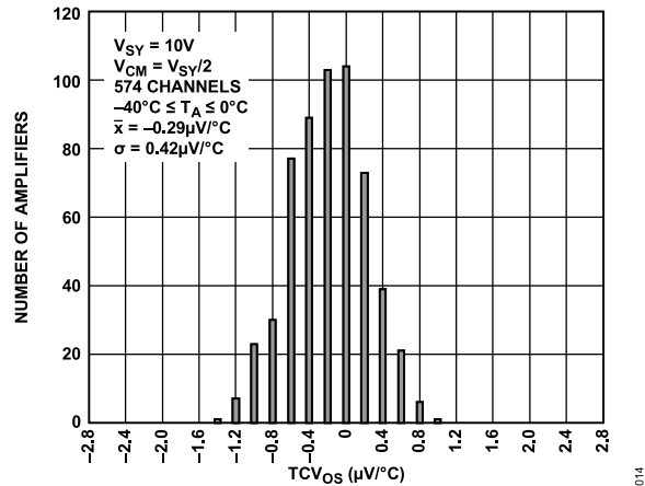
Figure 11. Input Offset Voltage Drift Distribution, -40^{\circ}\text{C} \leq T_A \leq 0^{\circ}\text{C} , V_{SY} = 10 V
