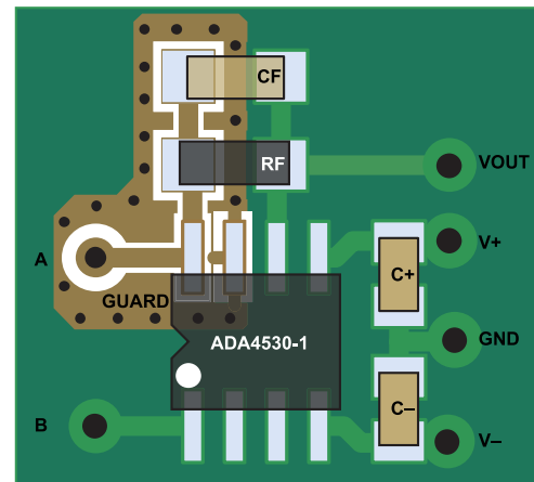
Figure 122. TIA Circuit Layout
