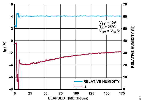
Figure 113. Effective Input Bias Current Transient Response to Humidity Step
