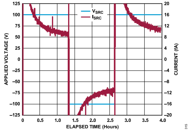
Figure 110. Glass Epoxy Dielectric Relaxation Performance
