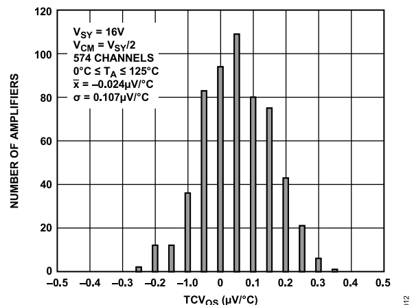
Figure 15. Input Offset Voltage Drift Distribution, 0^{\circ}\text{C} \leq T_A \leq 125^{\circ}\text{C} , V_{SY} = 16 V
