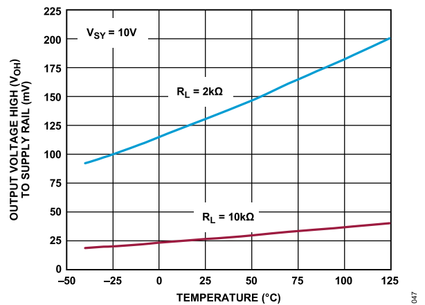
Figure 50. Output Voltage High ( V_{OH} ) to Supply Rail vs. Temperature, V_{SY} = 10\text{ V}
