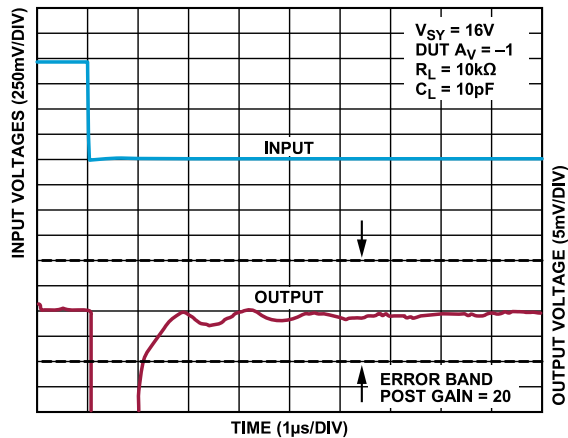
Figure 75. Negative Settling Time to 0.1%, V_{SY} = 16V
