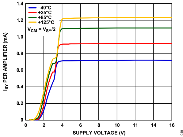
Figure 52. Supply Current ( I_S ) per Amplifier vs. Supply Voltage ( V_S )
