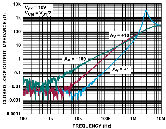
Figure 59. Closed-Loop Output Impedance vs. Frequency
