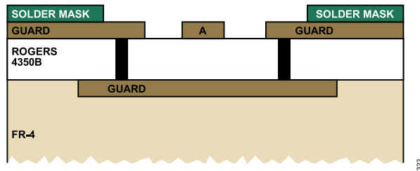
Figure 123. Layout Cross Section with Guard Plane
