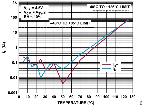
Figure 34. Input Bias Current ( I_B ) vs. Temperature, V_{SY} = 4.5\text{ V}
