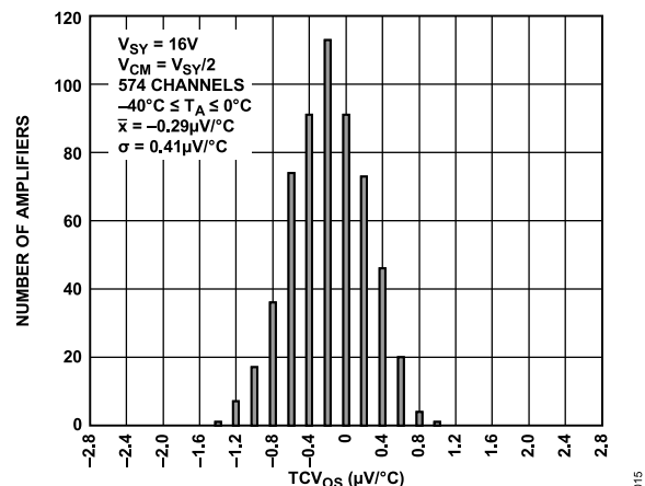
Figure 12. Input Offset Voltage Drift Distribution, -40^{\circ}\text{C} \leq T_A \leq 0^{\circ}\text{C} , V_{SY} = 16 V
