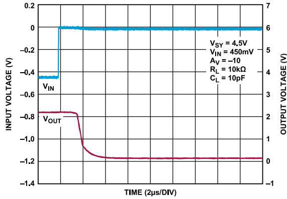
Figure 67. Positive Overload Recovery, V_{SY} = 4.5\text{ V}
