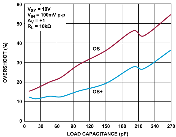
Figure 60. Small Signal Overshoot vs. Load Capacitance
