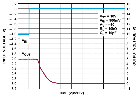
Figure 68. Positive Overload Recovery, V_{SY} = 10\text{ V}
