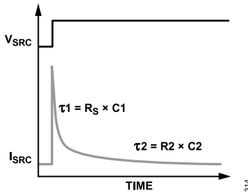
Figure 109. Step Response of Dielectric Relaxation Model
