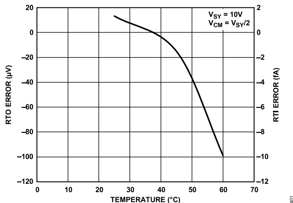
Figure 128. DC Error vs. Temperature
