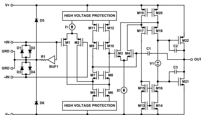
Figure 99. Simplified Schematic
