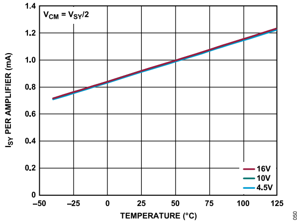
Figure 53. Supply Current ( I_S ) per Amplifier vs. Temperature
