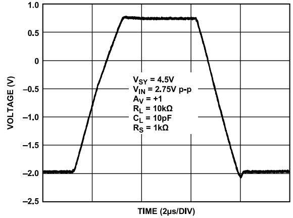
Figure 64. Large Signal Transient Response, V_{SY} = 4.5\text{ V}
