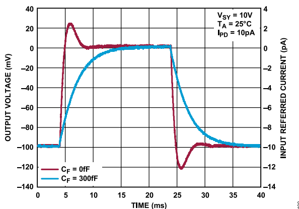
Figure 130. 10 pA Step Response
