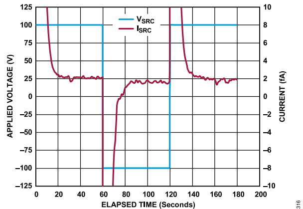
Figure 111. Rogers 4350B Dielectric Relaxation Performance
