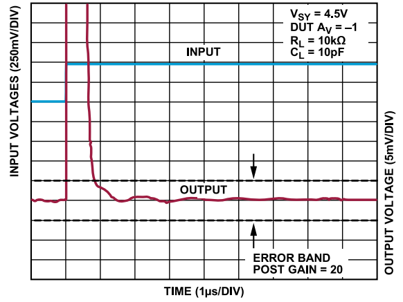
Figure 76. Positive Settling Time to 0.1%, V_{SY} = 4.5V
