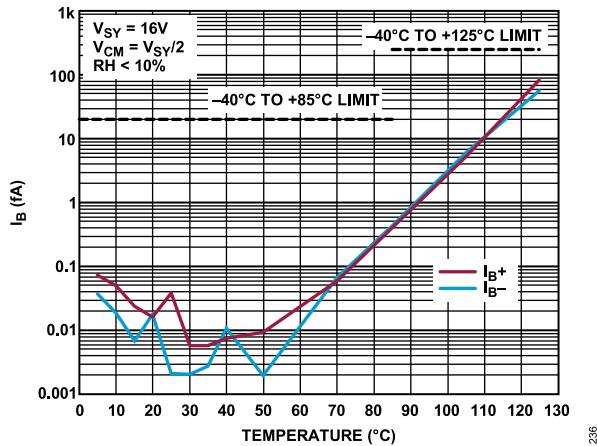
Figure 36. Input Bias Current ( I_B ) vs. Temperature, V_{SY} = 16\text{ V}
