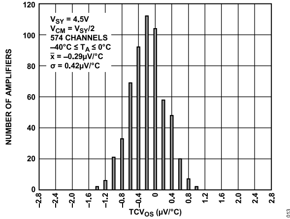
Figure 10. Input Offset Voltage Drift Distribution, -40^{\circ}\text{C} \leq T_A \leq 0^{\circ}\text{C} , V_{SY} = 4.5 V
