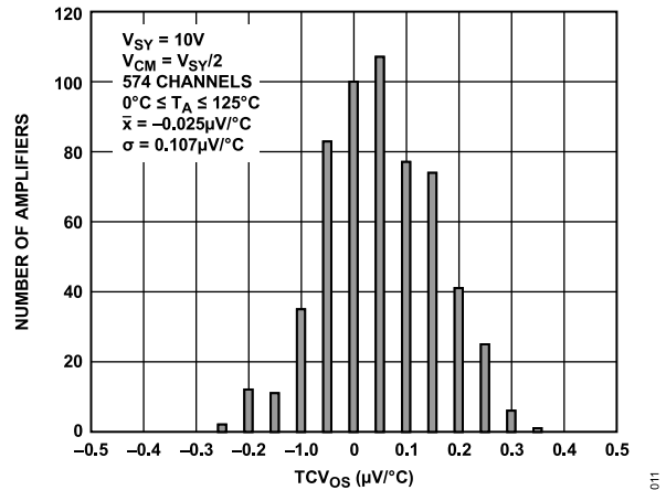
Figure 14. Input Offset Voltage Drift Distribution, 0^{\circ}\text{C} \leq T_A \leq 125^{\circ}\text{C} , V_{SY} = 10 V
