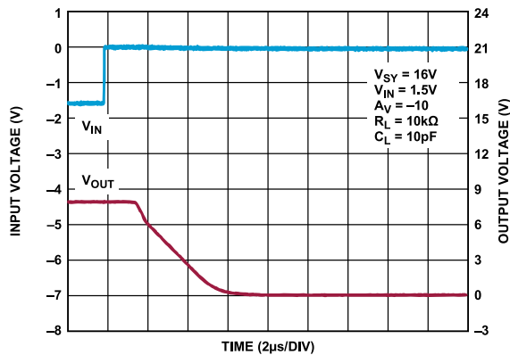
Figure 69. Positive Overload Recovery, V_{SY} = 16\text{ V}
