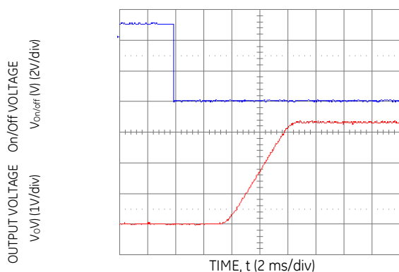
Figure 15. Typical Start-Up Using Remote On/Off with Low-ESR external capacitors (7x150µF Polymer) ( V_{in} = 5 Vdc, V_o = 3.3 Vdc, I_o = 5.0 A, C_o = 1050 µF).
