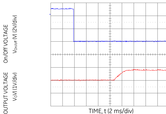
Figure 17 Typical Start-Up using Remote On/off with Prebias ( V_{in} = 3.3 Vdc, V_o = 1.8 Vdc, I_o = 1 A, V_{bias} = 1.0 Vdc).
