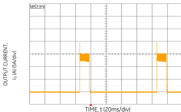
Figure 18. Output short circuit Current ( V_{in} = 5 Vdc, V_o = 0.75 Vdc).
