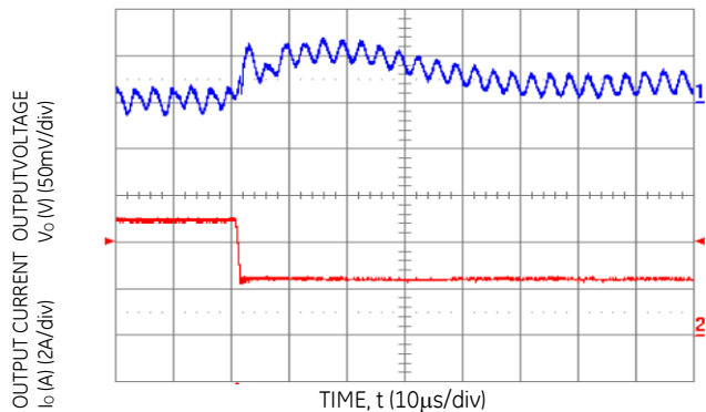
Figure 13. Transient Response to Dynamic Load Change from 100% of 50% full load ( V_o = 3.3 Vdc, C_{ext} = 2 \times 150 µF Polymer Capacitors).
