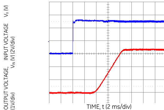
Figure 16. Typical Start-Up with application of V_{in} with ( V_{in} = 5.0 Vdc, V_o = 3.3 Vdc, I_o = 5 A).
