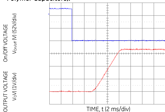
Figure 14. Typical Start-Up Using Remote On/Off ( V_{in} = 5 Vdc, V_o = 3.3 Vdc, I_o = 5.0 A).
