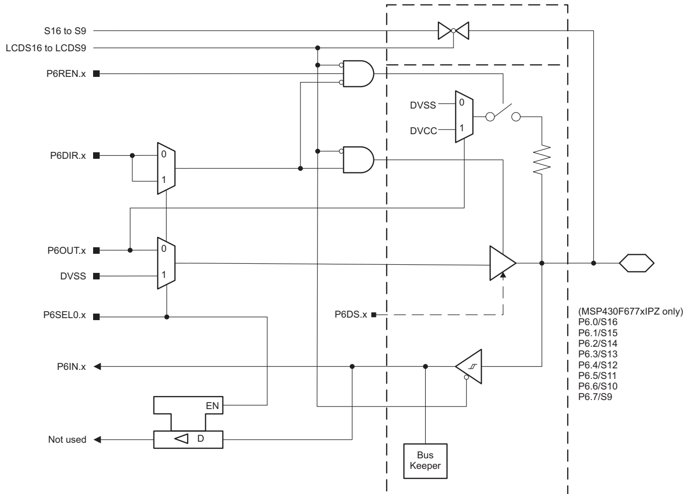
Figure 6-26. Port P6 (P6.0 to P6.7) Diagram (MSP430F677xIPZ Only)
