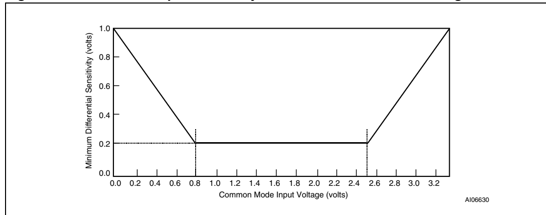
Figure 44. Differential input sensitivity over entire common mode range
