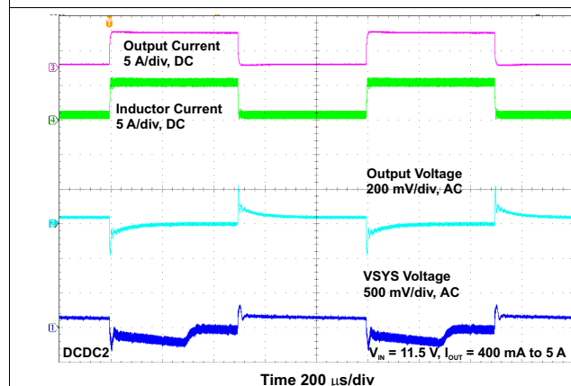
Figure 47. Load Transient Response
