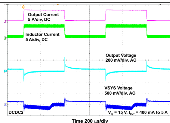
Figure 48. Load Transient Response
