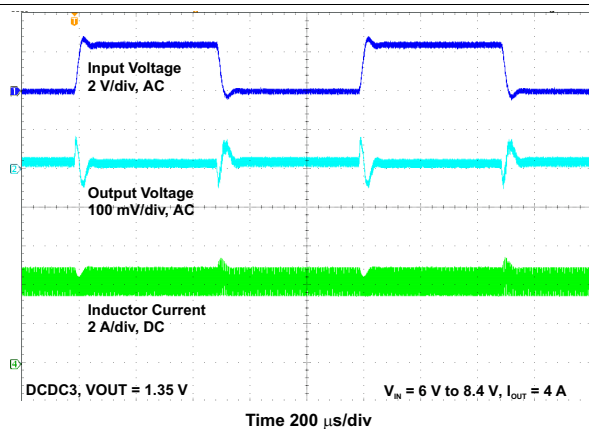
Figure 53. Line Transient Response
