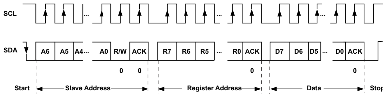
Figure 44. I²C Interface WRITE to in F/S Mode
