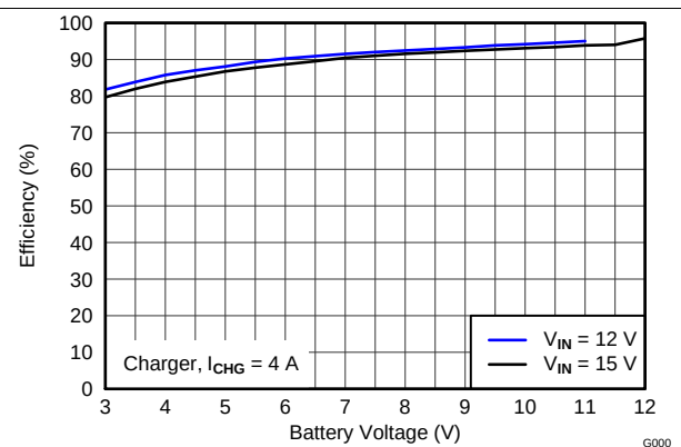
Figure 21. Efficiency vs Battery Voltage
