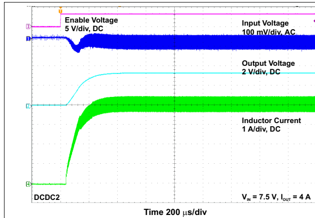
Figure 57. Start-Up After Enable
