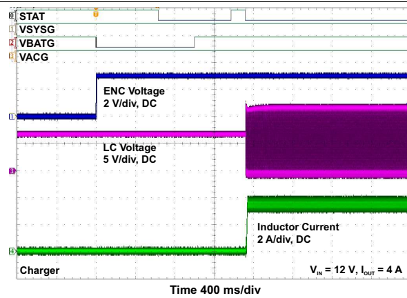
Figure 57. Start-Up After Enable
