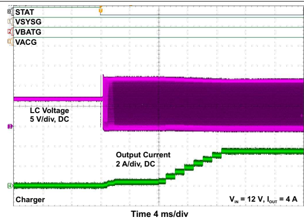
Figure 58. Start-Up After Enable
