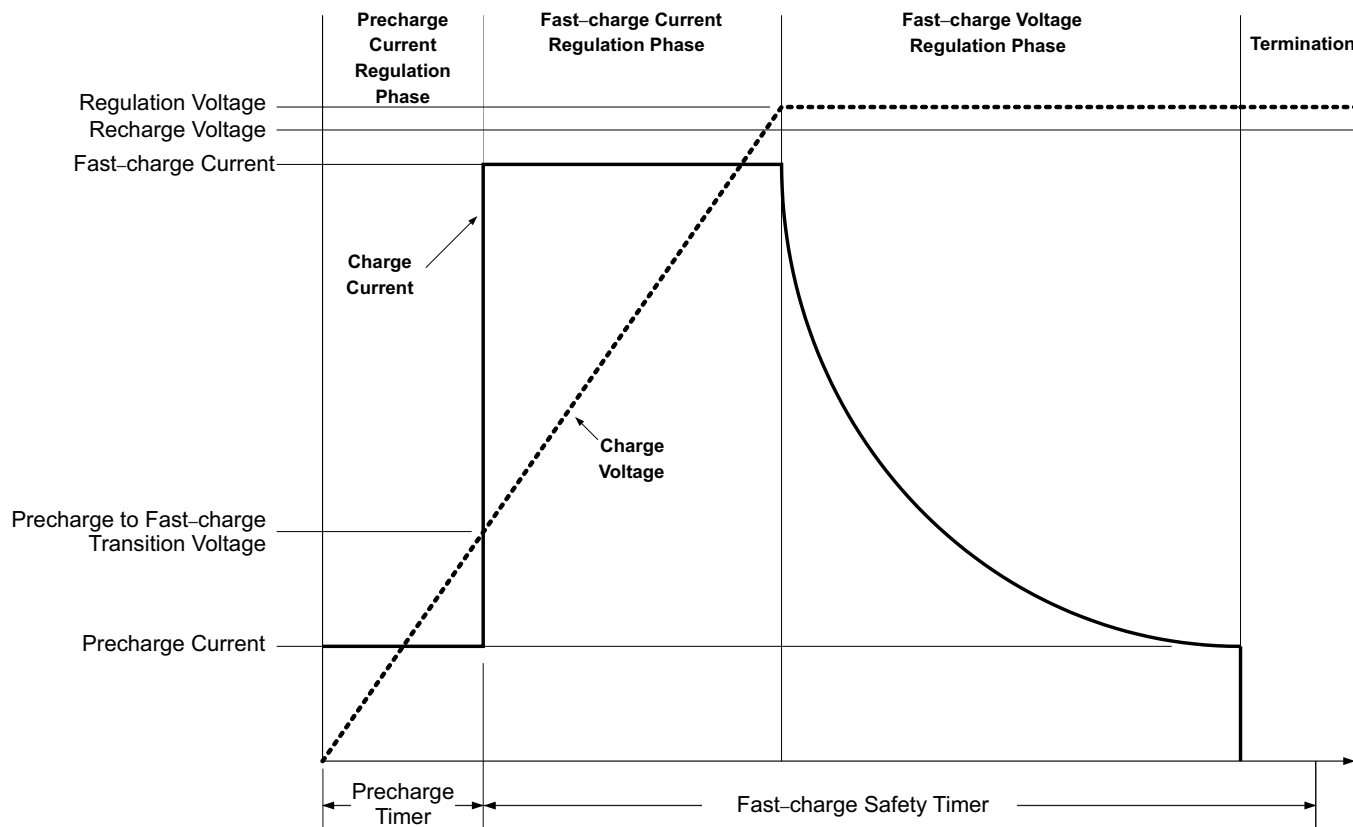
Figure 37. Charging Cycle
