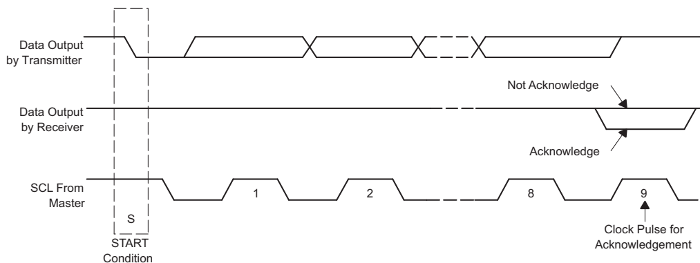
Figure 42. Acknowledge on the I²C-Bus
