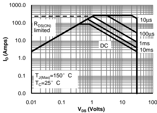
VGS > or equal 4.5V Figure 9: Maximum Forward Biased Safe Operating Area (Note F)
