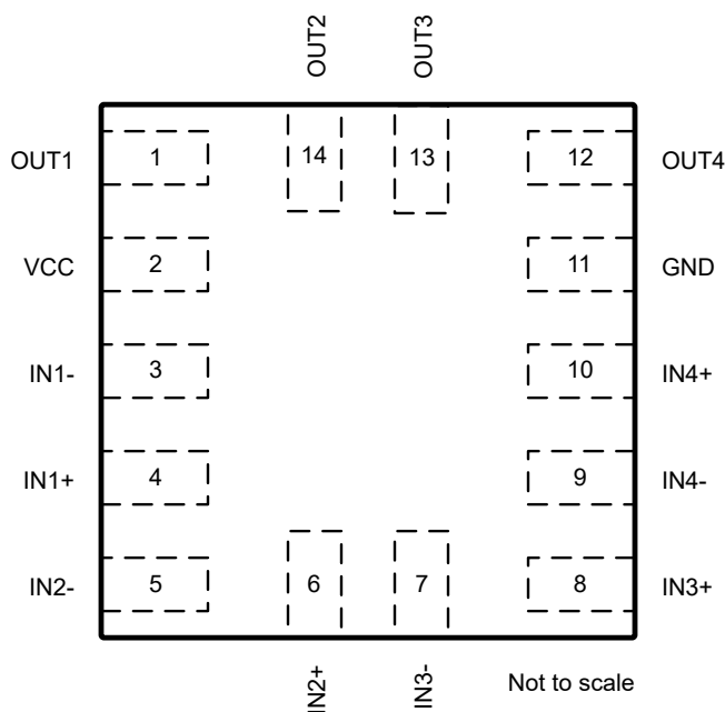
Figure 5-3. RUC Package 14-Pad X2QFN Top View
