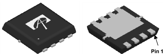
DFN 3x3 EP Top View Bottom View
