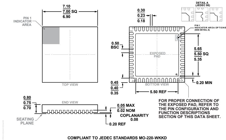
COMPLIANT TO JEDEC STANDARDS MO-220-WKKD Figure 85. 48-Lead Lead Frame Chip Scale Package [LFCSP] 7 mm x 7 mm Body and 0.75 mm Package Height (CP-48-9) Dimensions shown in millimeters
