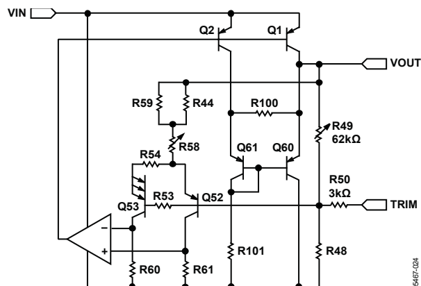
Figure 36. Simplified Schematic
