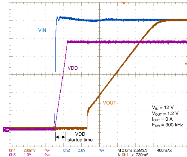
Figure 25. Typical Startup Waveforms of VDD and VOUT With Controlled Ramp Rates
