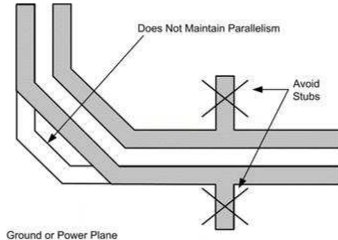
Figure 36. Avoiding Stubs in a Differential Signal Pair
