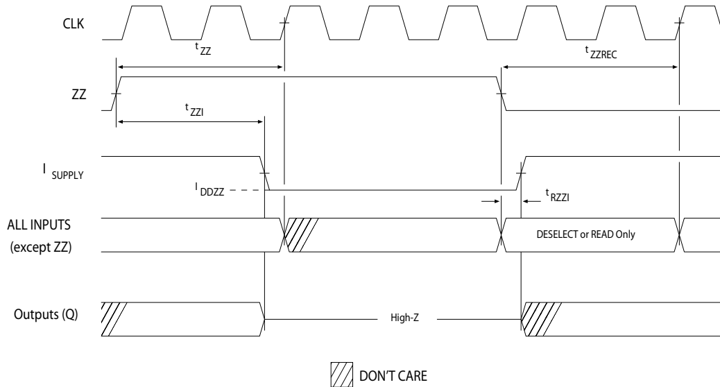
Figure 8. ZZ Mode Timing [37, 38]
