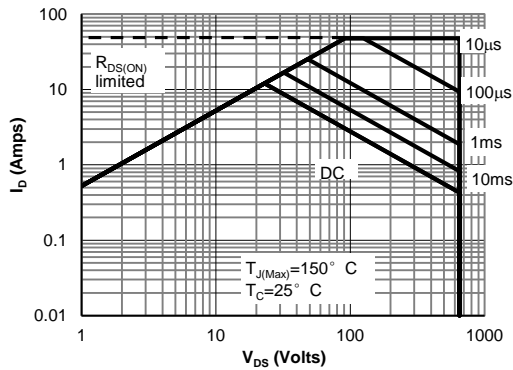
Figure 9: Maximum Forward Biased Safe Operating Area for AOT(B)12N65(L) (Note F)
