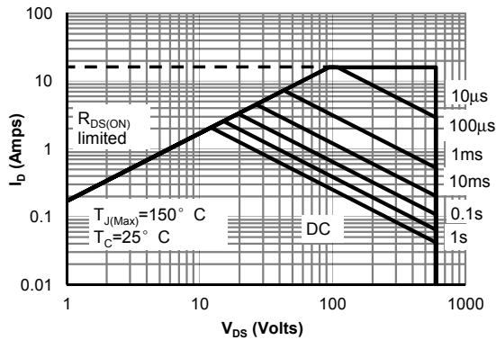
Figure 11: Maximum Forward Biased Safe Operating Area for AOTF4N60L (Note F)
