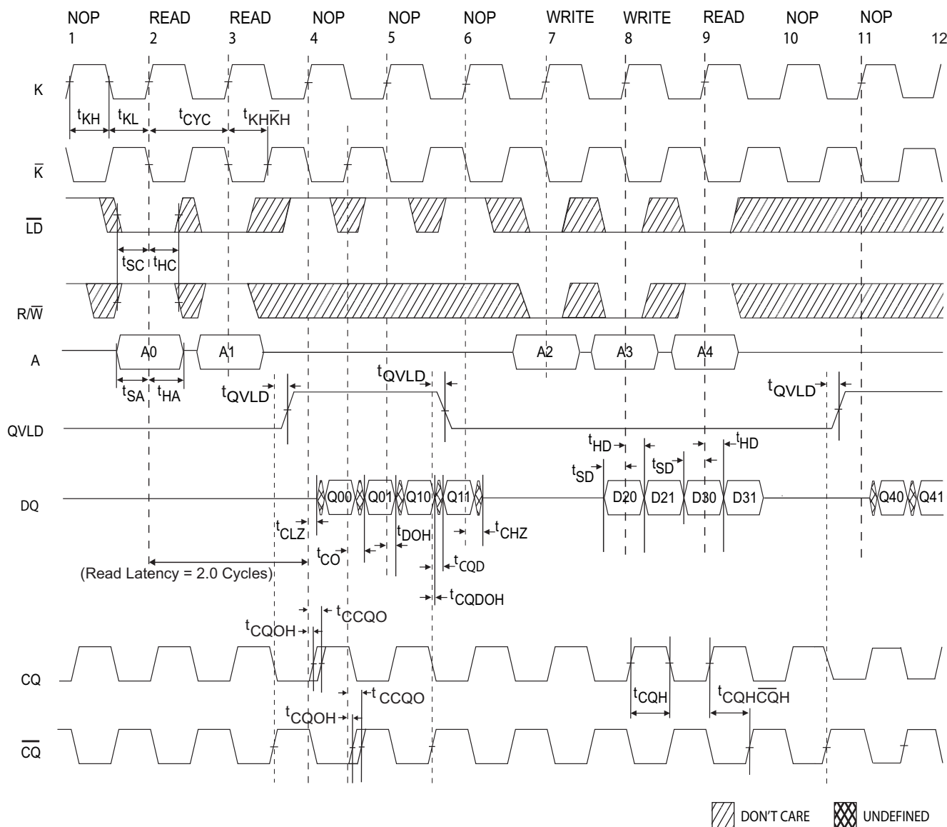
Figure 5. Waveform for 2.0 Cycle Read Latency
