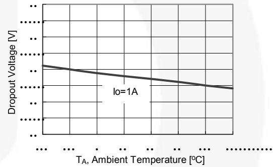
Figure 5. Dropout Voltage
