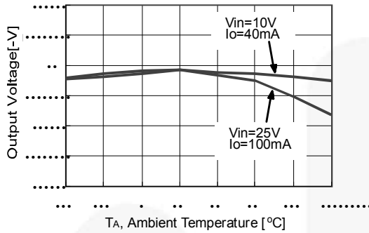
Figure 2. Output Voltage
