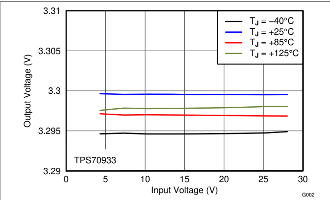
Figure 6-2. 3.3-V Line Regulation vs V_{IN} and Temperature
