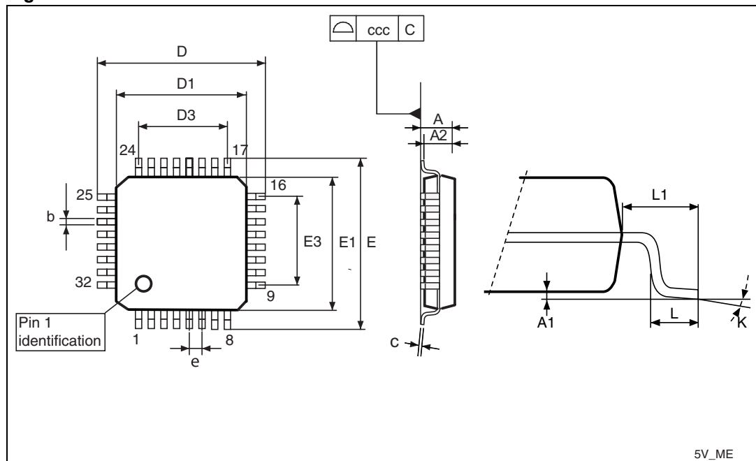
Figure 11. LQFP32 outline
