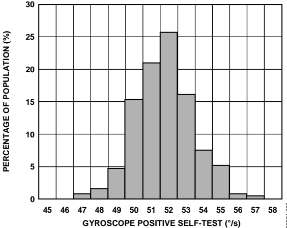
Figure 21. Gyroscope Positive Self-Test Distribution, +25°C
