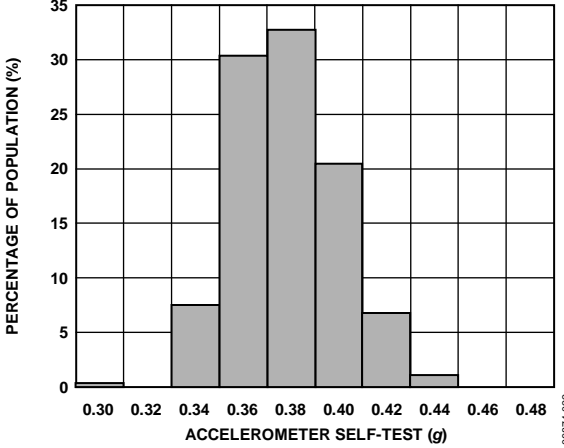
Figure 23. Accelerometer Self-Test Distribution, +25°C
