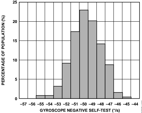
Figure 22. Gyroscope Negative Self-Test Distribution, +25°C
