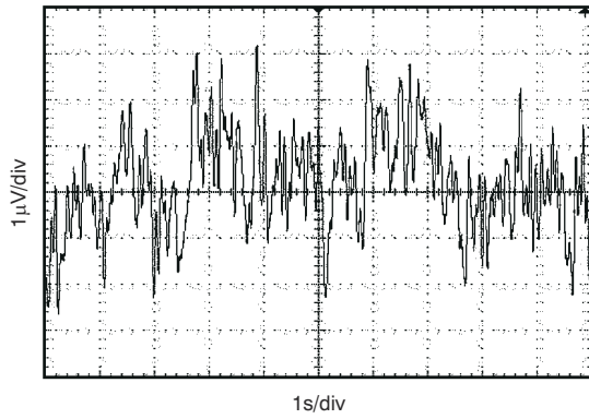
Figure 7-13. 0.1 Hz to 10 Hz Noise
