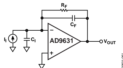
Figure 61. Transimpedance Configuration
