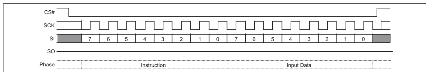
Figure 71 Write VDLR (WVDLR) command sequence
