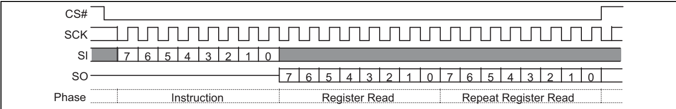
Figure 58 Read Configuration Register (RDCR) command sequence
