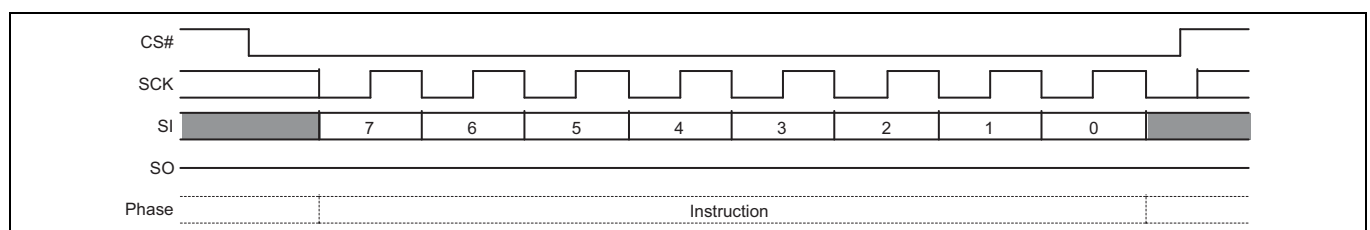
Figure 110 PPB Erase command sequence
