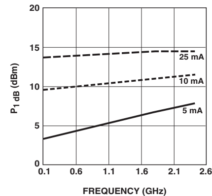
Figure 8. AT-41511 and AT-41533 P_{1dB} vs. Frequency and Bias at V_{CE} = 5 V, with Optimal Tuning.
