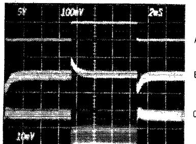
MAX741U LOAD-TRANSIENT RESPONSE
