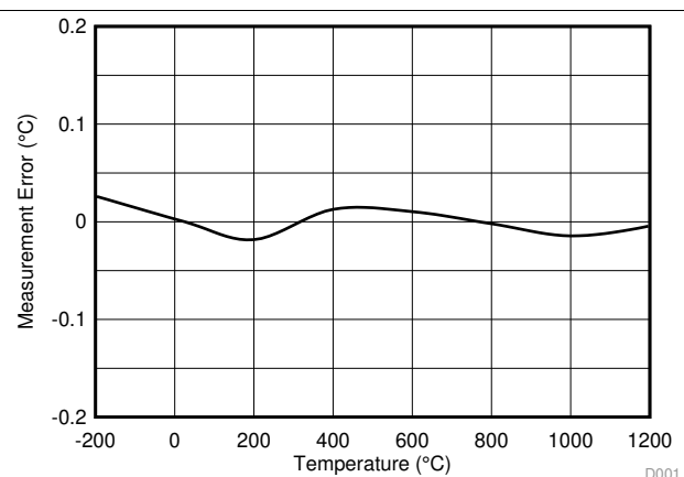
Figure 76. Temperature Measurement Error vs T_{(TC)}
