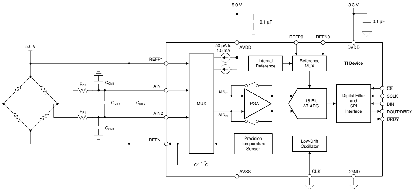
Figure 82. Bridge Measurement
