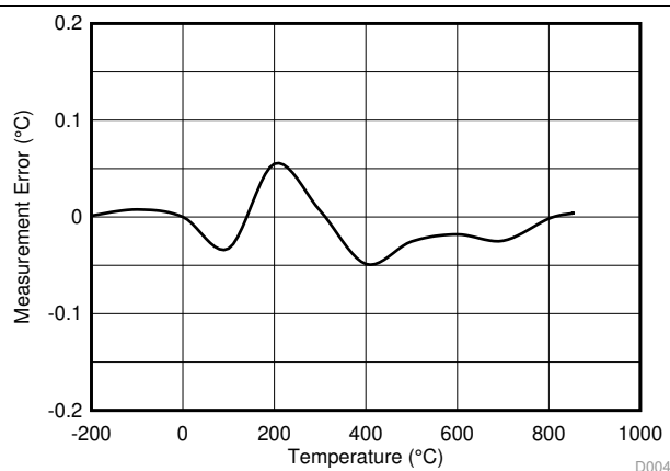
Figure 81. Temperature Measurement Error vs T_{(\text{RTD})}
