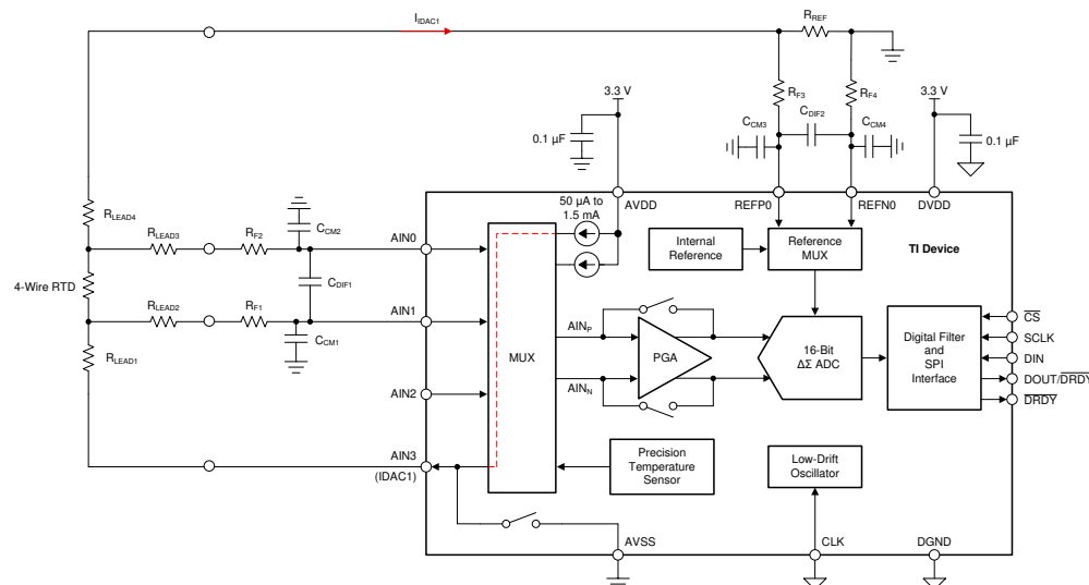
Figure 79. 4-Wire RTD Measurement
