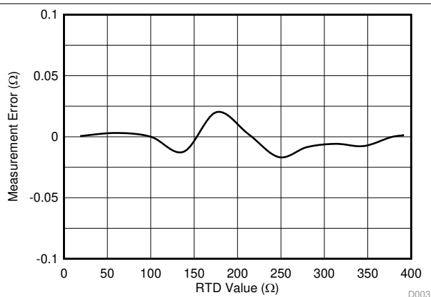
Figure 80. Resistance Measurement Error vs R_{\text{RTD}}
