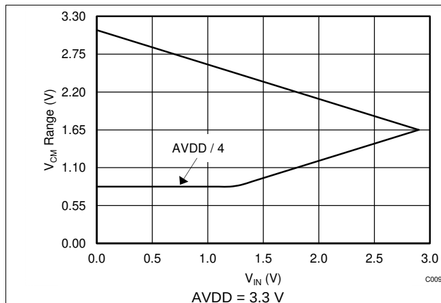
Figure 41. Common-Mode Voltage Limits (Gain = 1)
