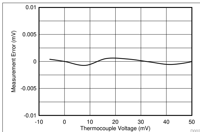
Figure 75. Voltage Measurement Error vs V_{(TC)}
