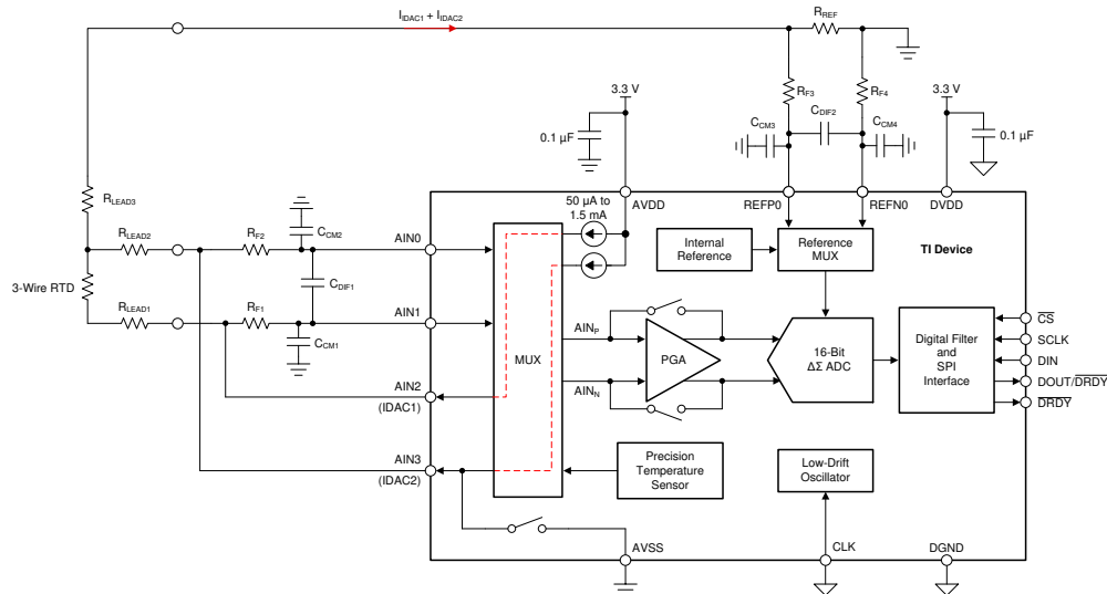
Figure 77. 3-Wire RTD Measurement
