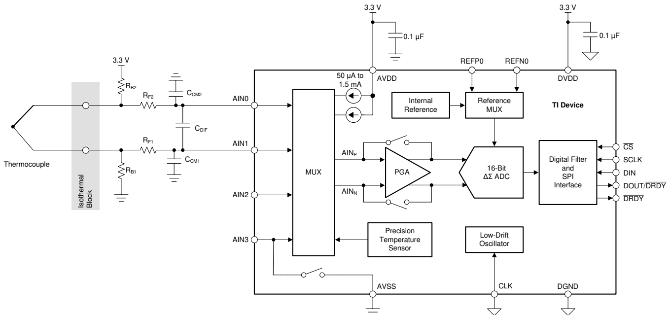
Figure 74. Thermocouple Measurement
