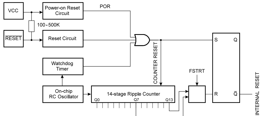
Figure 23. Reset Logic
