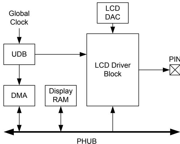
Figure 8-9. LCD System
