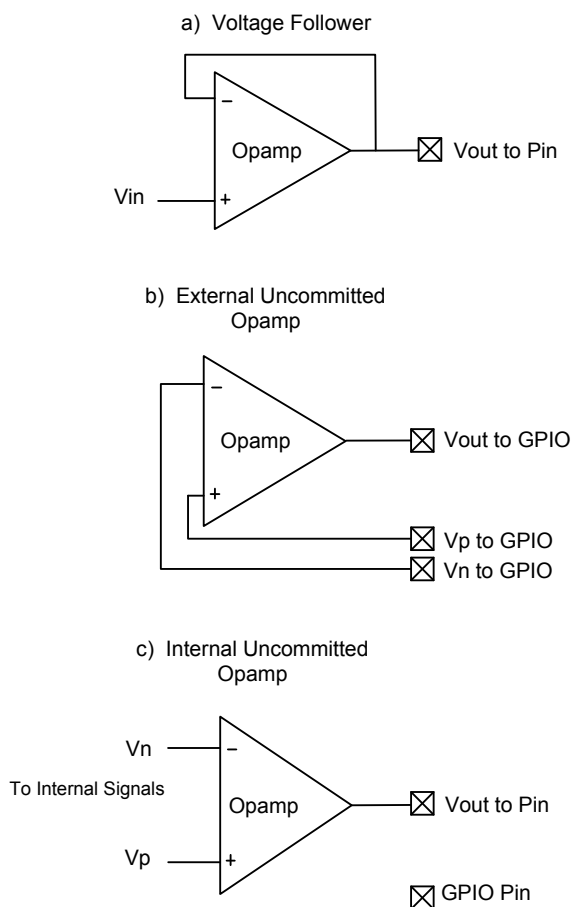
Figure 8-6. Opamp Configurations
