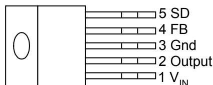
TO220-5L
