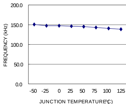
Switch Frequency
