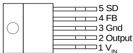
TO220-5/TO220-5 (R)
