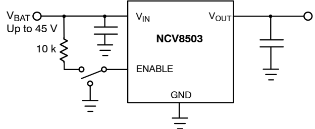
Figure 17. ENABLE Function
