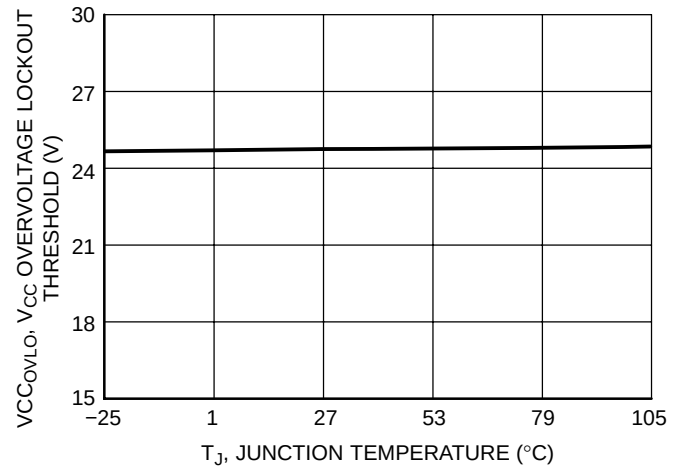
Figure 22. V_{CC} Overvoltage Lockout Threshold vs. Junction Temperature
