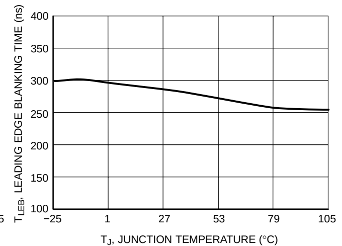
Figure 8. Leading Edge Blanking Time vs. Junction Temperature
