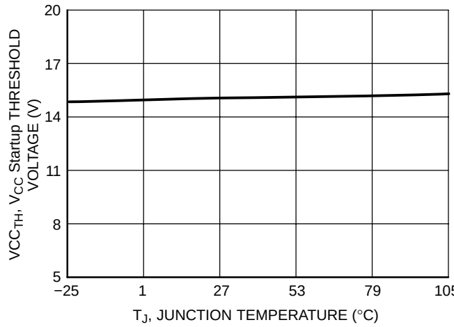
Figure 23. V_{CC} Startup Threshold Voltage vs. Junction Temperature
