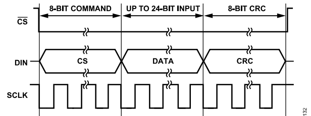
Figure 123. SPI Write Transaction with CRC
