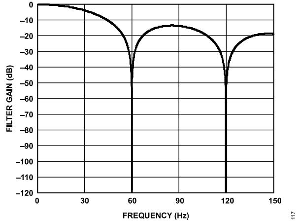
Figure 108. 60 Hz Rejection
