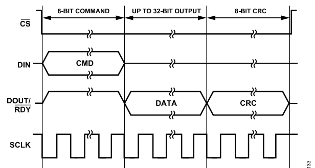
Figure 124. SPI Read Transaction with CRC
