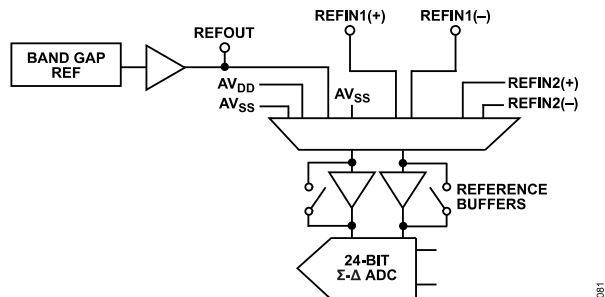
Figure 76. Reference Connections
