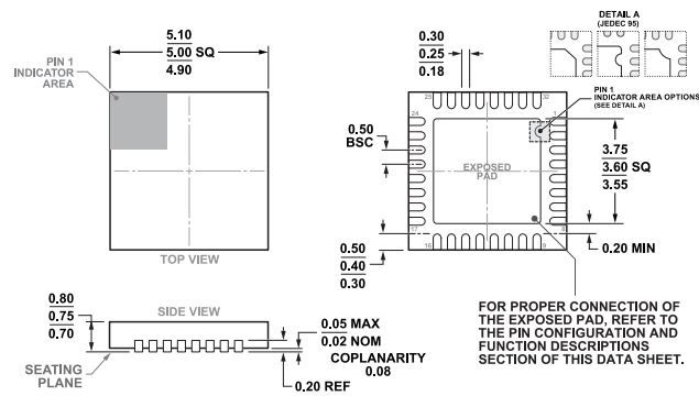
Figure 130. 32-Lead Lead Frame Chip Scale Package [LFCSP] 5 mm × 5 mm Body and 0.75 mm Package Height (CP-32-12) Dimensions shown in millimeters
