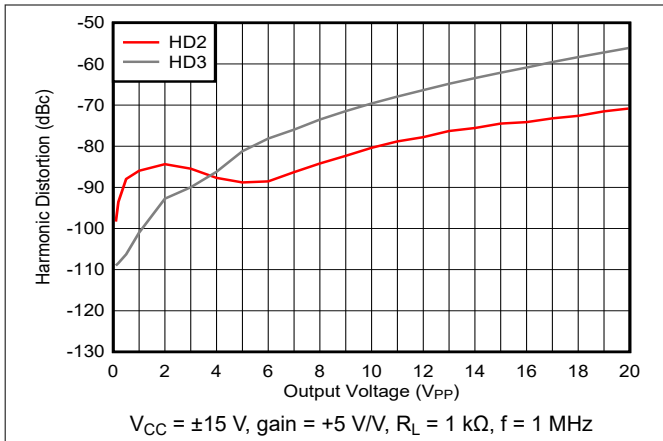
Figure 5-19. Harmonic Distortion vs Peak-to-Peak Output Voltage
