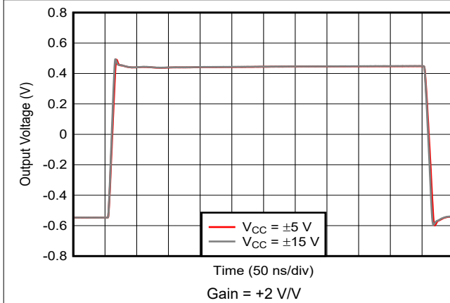
Figure 5-21. 1-V Step Response
