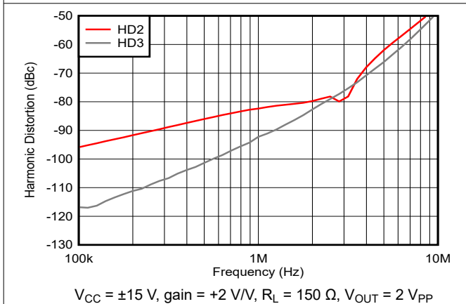
Figure 5-17. Harmonic Distortion vs Frequency
