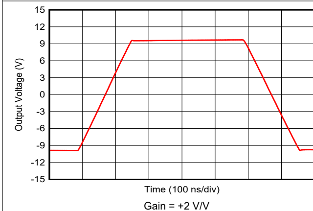
Figure 5-23. 20-V Step Response
