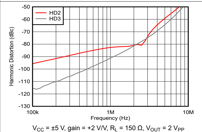
Figure 5-18. Harmonic Distortion vs Frequency
