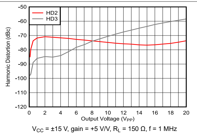
Figure 5-20. Harmonic Distortion vs Peak-to-Peak Output Voltage
