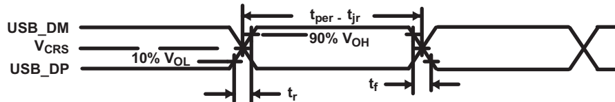
Figure 5-34. USB2.0 Integrated Transceiver Interface Timing
