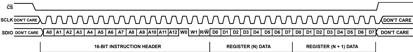
Figure 50. Serial Control Port Write—LSB First, 16-Bit Instruction, Two Bytes of Data
