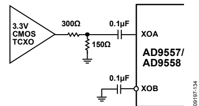
Figure 34. System Clock Input (XOA, XOB) when Using a TCXO/OCXO with 3.3 V CMOS Output
