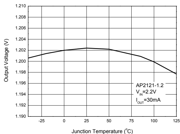
Figure 13. Output Voltage vs. Junction Temperature
