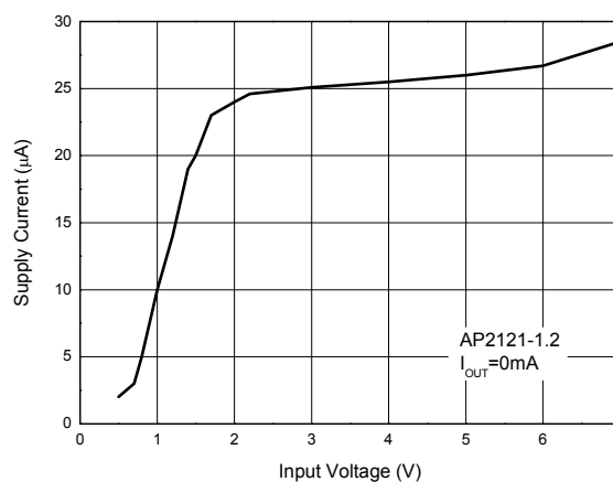
Figure 15. Supply Current vs. Input Voltage
