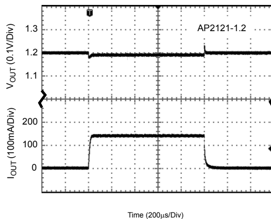
Figure 21. Load Transient (Conditions: V_{IN}=2.2\text{V} , C_{IN}=1\mu\text{F} , C_{OUT}=1\mu\text{F} )
