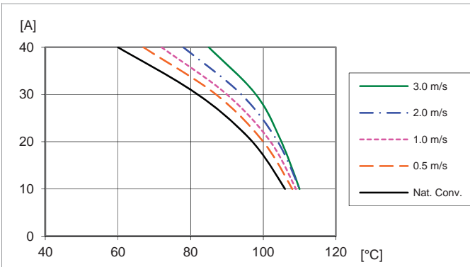
Available load current vs. ambient air temperature and airflow at V_0 = 1.0\text{ V} , V_i = 12\text{ V} . See Thermal Consideration section.
