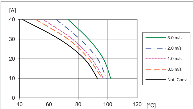
Available load current vs. ambient air temperature and airflow at V_0 = 3.3\text{ V} , V_i = 12\text{ V} . See Thermal Consideration section.
