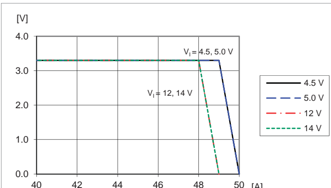
Output voltage vs. load current at T_{pj} = +25\text{ °C} , V_0 = 3.3\text{ V} . Note: Output enters hiccup mode at current limit.
