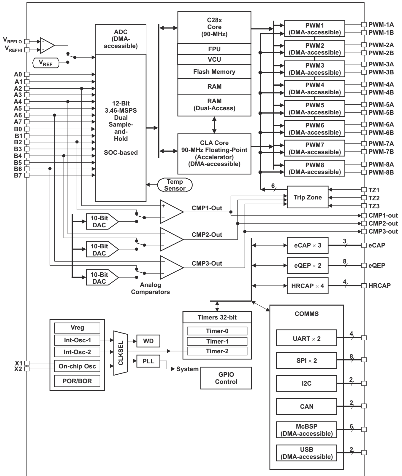
Figure 3-2. Peripheral Blocks
